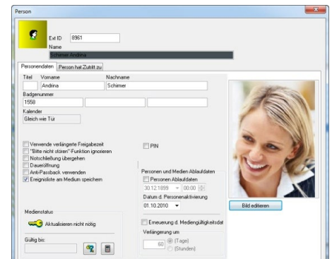
Software
